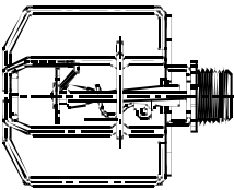
MODEL G HORIZONTAL SIDE WALL
