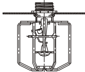
MODEL GFR 3/4" NPT PENDENT INTERMEDIATE
