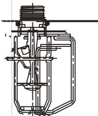
EL GFR 1/2" NPT PENDENT INTERMEDIATE
