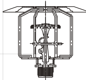
MODEL G UPRIGHT
