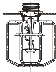
MODEL G 3/4" NPT PENDENT INTERMEDIATE
