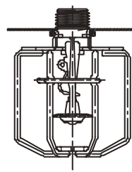
MODEL G 1/2" NPT PENDENT INTERMEDIATE
